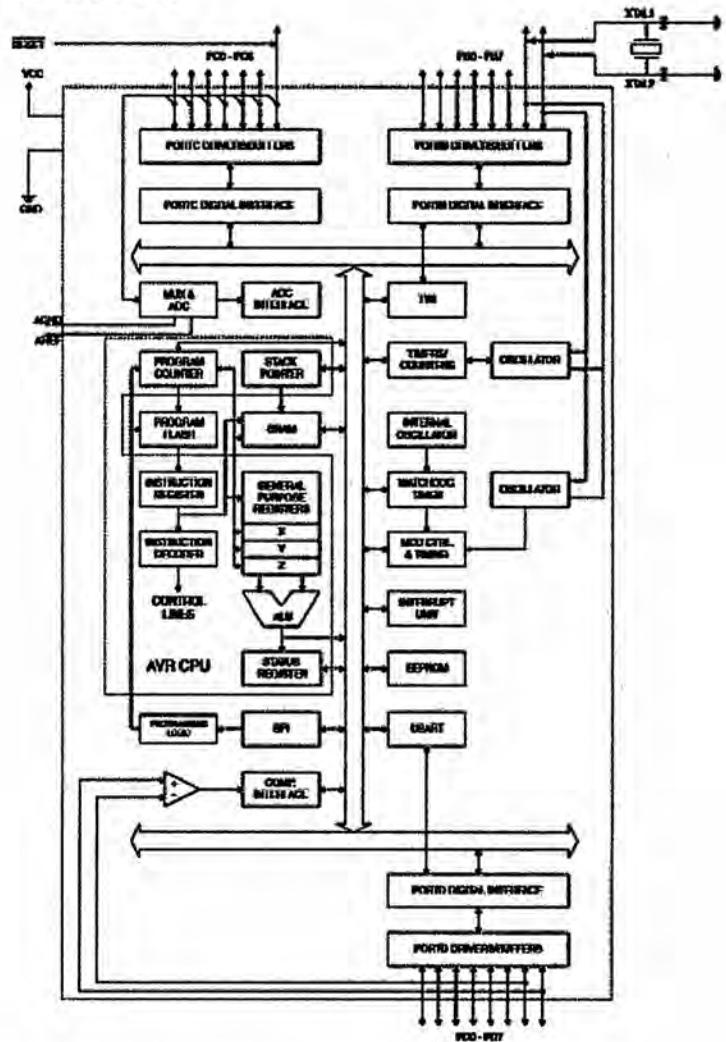
Figure 1. Block Diagram
