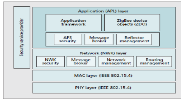
■ Figure 1. ZigBee stack diagram.
